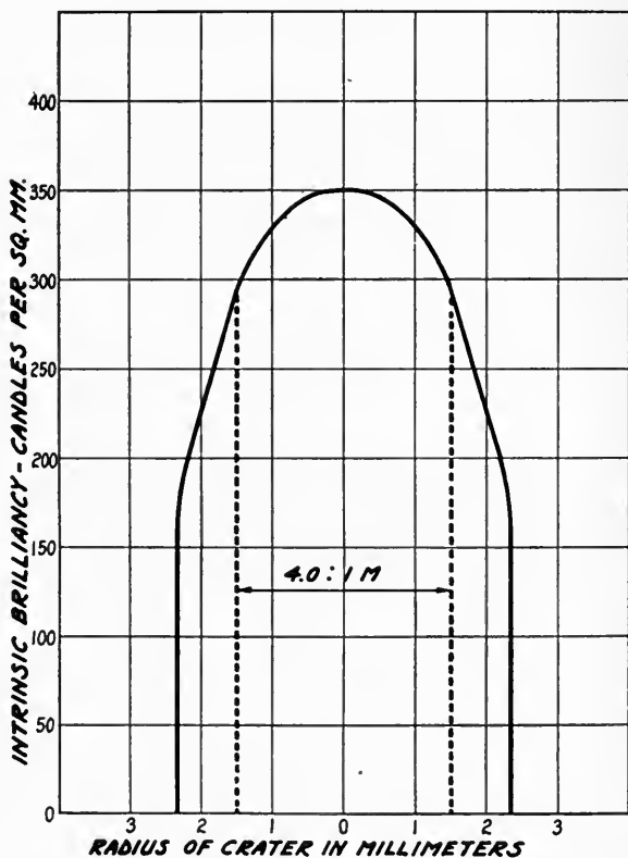
FIG. 2. Intrinsic brilliancy across positive crater with 6-mm "National" "Pearlex" Positive—5.5-mm "National" "Pearlex" Negative at 30 amperes, 28 volts d-c.
